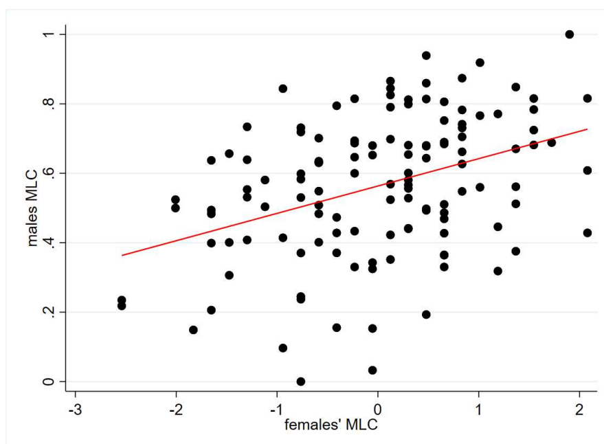
Figure 1. Scatter plot of the association between males' and females' MLC
