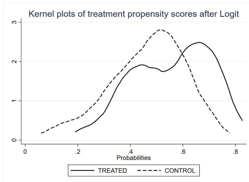
Figure 2. Kernel plots of treatment propensity scores after Logit
