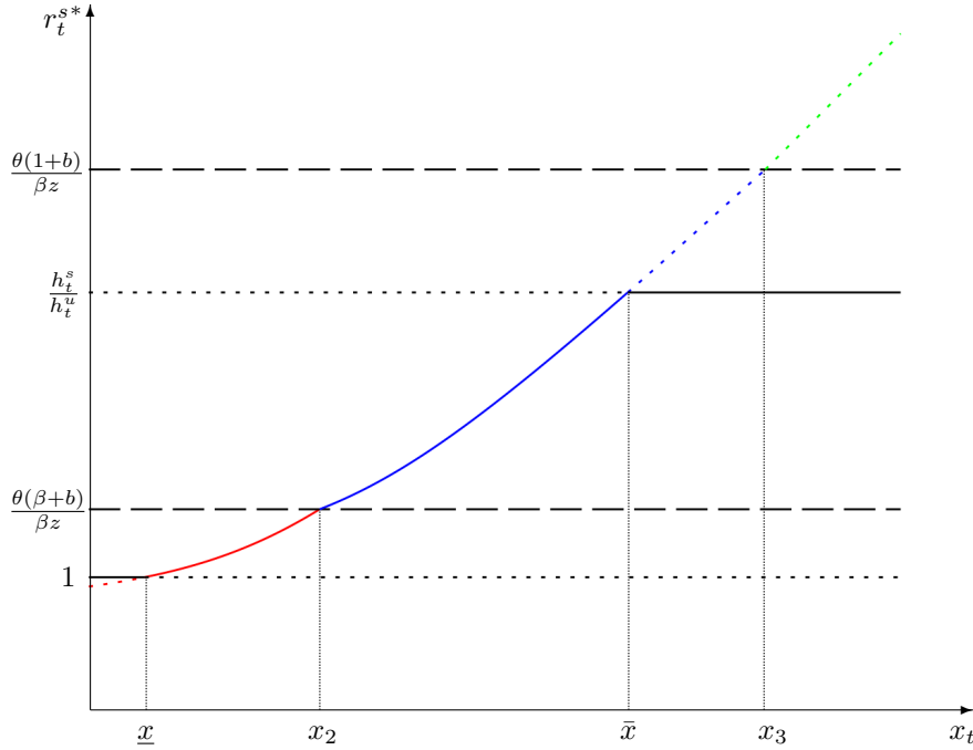
Figure 1: A numerical illustration of r_t^{s*} as a function of x_t . An internal equilibrium exists if, and only if, \underline{x} \leq x_t \leq \bar{x} . Value of parameters: \alpha = 0.9 ; \mu = 0.3 ; z := 0.3 ; \theta = 0.25 ; \beta = 0.4 ; b = 0.2 ; a = 1 .
